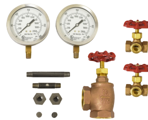
CHECKTRIM Riser Check Trim Kits
