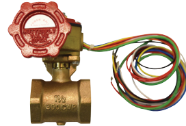
F49BR 1" - 2-1/2" Powerball Butterfly Valve Threaded Connections
