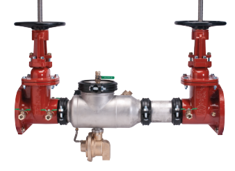
375ASTDAR 2-1/2" - 10" OSY (standard), PI or Butterfly (optional)
